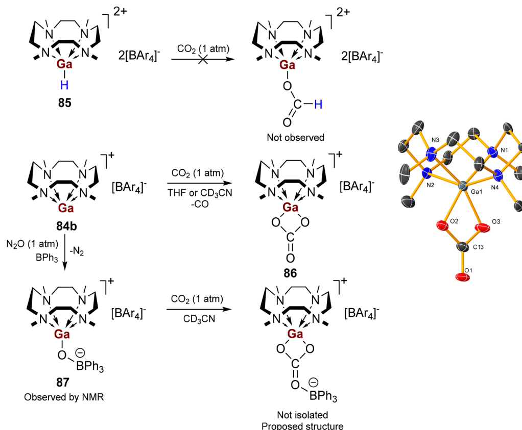
Scheme 35 Reactivity of 84b and 85 towards CO 2 and N 2 O (Ar = C 6 H 3 -3,5-Me 2 ). Cationic part of the crystal structure of 86 (H-atoms omitted). 124
