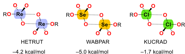
Scheme 2 Self-assembled dimers dictated by matere (HETRUT), 43 chalcogen (WABPAR) 44 and halogen (KUCRAD) 45 bonds. The dimerization energies are indicated.
