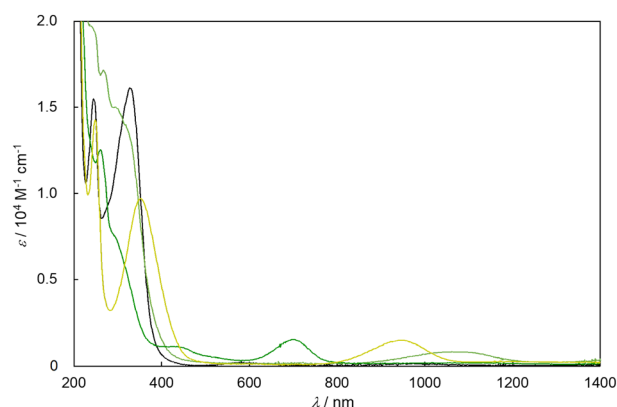
Fig. 4 UV-vis-NIR spectra of [\text{IV,IV}]^{2+} (green line), [\text{III,IV}]^+ (olive line), [\text{III,IV}_2\text{1H}]^{2+} (yellow-green line), and [\text{III,III}_2\text{2H}]^{2+} (black line) in \text{CH}_3\text{CN} .
