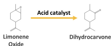
Scheme 3 Acid-catalyzed limonene oxide isomerization.
