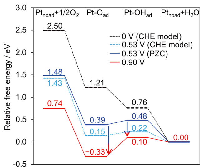
Fig. 2 Free energy profiles of the ORR in a vacuum using the CHE model at 0 V (black dash) and 0.53 V (aqua dash), at the potential of zero charge (pzc) of Pt noad (blue), and at 0.90 V vs. SHE (red).
