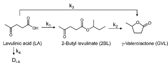
Scheme 2 Mechanistic proposal for LA conversion to GVL production, in 2BuOH at 180 °C.
