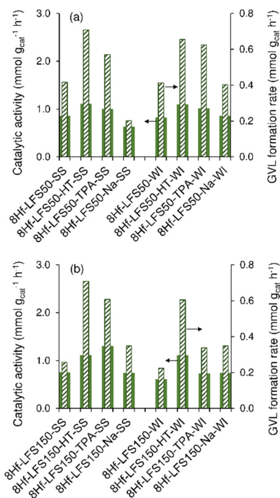
Fig. 9 Catalytic activity and GVL formation rate for the 8Hf-LFS50s (a) and 8Hf-LFS150s (b) prepared via the SS or WI impregnation method. Reaction conditions: 0.45 M LA in 2BuOH, 25.5 g cat L -1 , 180 °C.
