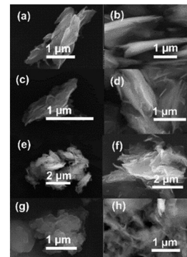
Fig. 5 SEM images of LFS50 (a), LFS150 (b), LFS50-HT (c), LFS150-HT (d), H-LFS50-TPA (e), H-LFS150-TPA (f), H-LFS50-Na (g), and H-LFS150-Na (h).
