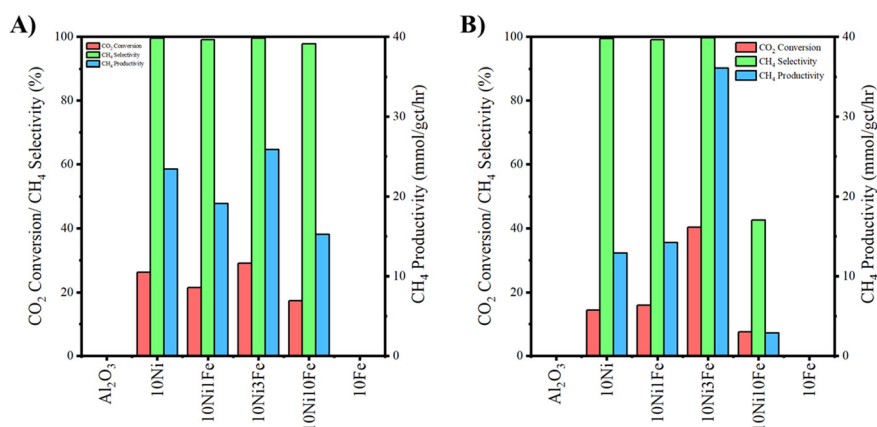
Fig. 6 CO 2 conversion and CH 4 selectivity during thermal-catalytic CO 2 methanation at 300 °C by 10Ni, 10Fe and 10Ni x Fe (where x = 1, 3, 10) Al 2 O 3 -supported catalysts. Neat Al 2 O 3 is included as a control. Where: A) WI; B) DP.
