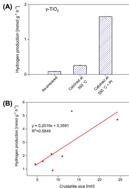
Fig. 2 (A) Hydrogen production rate of the prepared \gamma\text{-TiO}_2 catalysts and (B) relationship between crystalline size and hydrogen production.
