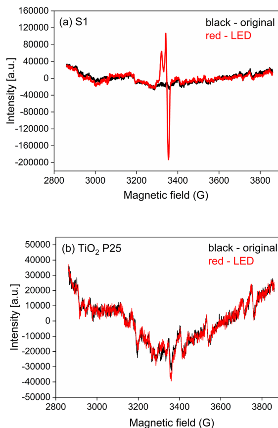
Fig. 12 EPR spectra of (a) S1 – yellow \text{TiO}_2 synthesized with PVP as a stabilizer, and (b) white commercial \text{TiO}_2 P25.
