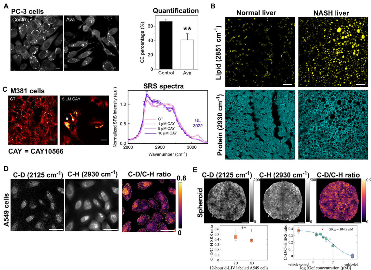
Fig. 7 Visualising drug-cell interactions and phenotypic outcomes using SRS microscopy. (A) SRS images of PC-3 cells treated with avasimibe (5 \mu\text{mol L}^{-1} , 3 days) vs. control cells. Scale bar: 10 \mu\text{m} . Quantification of the cholesterol ester (CE) percentage is also presented. Images reproduced from ref. 96 with permission from American Association for Cancer Research. 96 Copyright 2018. (B) Decomposed images of lipid (2850 \text{cm}^{-1} ), and protein (2930 \text{cm}^{-1} ) of a normal liver (HH1142) and a non-alcoholic steatohepatitis (NASH) liver (UMN1249). Scale bars: 50 \mu\text{m} . Images reproduced from ref. 105 with permission from Nature Publishing Group. 105 Copyright 2018. (C) SRS imaging of melanoma cell line exposed to DMSO (control, CTL) or CAY10566 (a SCD1 ( \Delta 9 -desaturase inhibitor)). Hyperspectral SRS imaging shows a decrease in unsaturated lipid (UL) content at 3022 \text{cm}^{-1} with increasing [CAY10566]. Images reproduced from ref. 113 with permission from Nature Publishing Group. 113 Copyright 2020. (D) Live A549 cells were treated with lapatinib (5 \mu\text{M} , 24 h) before d-LIV (6 h). SRS images were acquired at 2125 \text{cm}^{-1} (C–D region) and 2930 \text{cm}^{-1} (C–H region). Ratiometric imaging was used to demonstrate the response to lapatinib treatment. Images reproduced from ref. 117 with permission from American Chemical Society. 117 Copyright 2024. (E) Representative SRS images of the C–D and C–H region together with a ratiometric SRS image formed from A549 spheroids following a 12 h d-LIV labelling method. A comparison of the growth rate in the 2D and 3D cultures is also provided. Significance: **: p \leq 0.01 . Lastly, a comparison of the SRS ratio of C–D/C–H in an A549 spheroid following treatment with varying concentrations of gefitinib for 12 h using this method is provided. Scale bar: 50 \mu\text{m} . Image reproduced from ref. 118 with permission from American Chemical Society. 118 Copyright 2023.
