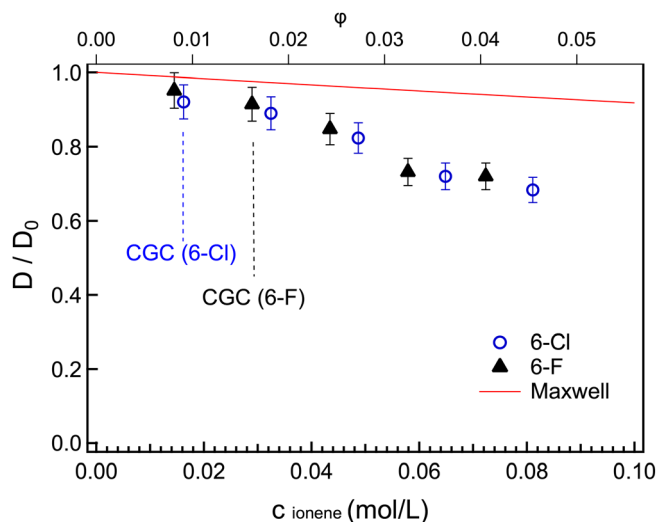
Fig. 9 Self-diffusion of water in 6-F and 6-Cl solutions and gels, normalised to the bulk self-diffusion coefficient of HDO contained in \text{D}_2\text{O} at 18 °C ( 1.64 \times 10^{-9} \text{ m}^2 \text{ s}^{-1} ). The secondary horizontal axis depicts the volume fraction ( \phi ) occupied by ionene (at 0.1 mol \text{L}^{-1} this corresponds to 5.6%) and serves to plot the prediction of the simple Maxwell obstruction model, for which D/D_0 = (1 - \phi)/(1 + \phi/2) . 46
