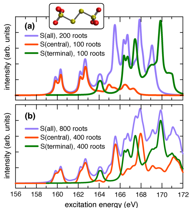
Fig. 6 XAS of (S_4O_6)^{2-} at the sulfur L-edge. All calculations were performed using CAM-B3LYP/CIS + SOC with def2-TZVPPD, computing either (a) 200 or (b) 800 singlet and triplet excited states, which were then broadened using a Lorentzian function (FWHM = 0.2 eV). Spectra labeled S(terminal) and S(central) employ only the S(2p) orbitals on the indicated atoms, with a correspondingly smaller number of excited states, whereas S(all) uses all of the S(2p) orbitals.
