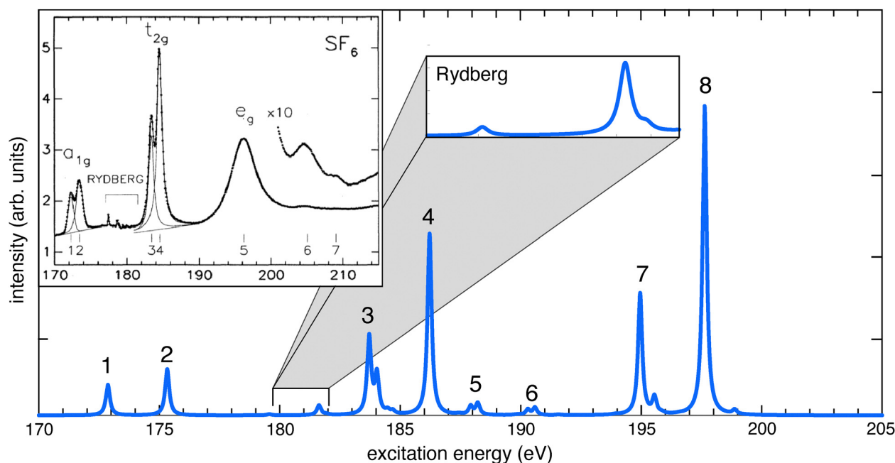
Fig. 7 L-edge XAS of SF_6 . The CAM-B3LYP/CIS + SOC spectrum (in blue) was obtained using the def2-TZVPPD basis set with 200 singlet and 200 triplet states. Individual transition energies were shifted by 5 eV and broadened with a Lorentzian function (FWHM = 0.3 eV). The experimental spectrum (inset) is reproduced from ref. 134; copyright 1993 American Physical Society.
