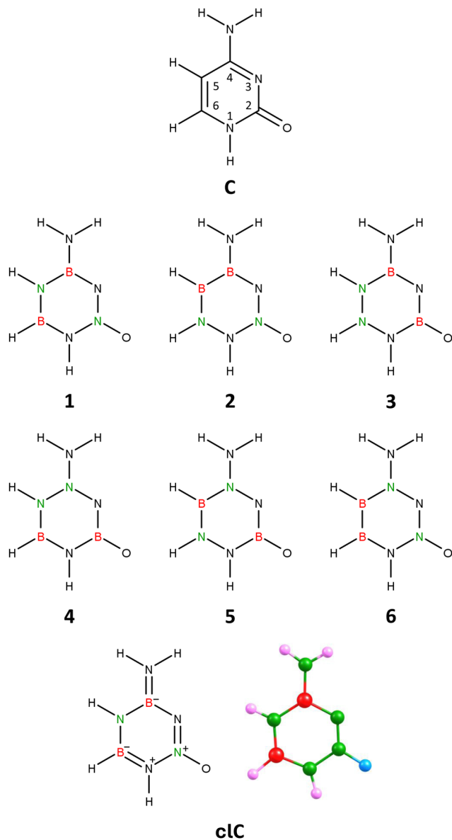
Fig. 1 Cytosine (C), isomers 1–6 of carbonless cytosine, and the equilibrium structure of the chosen cytosine equivalent (isomer 1), cIC.
