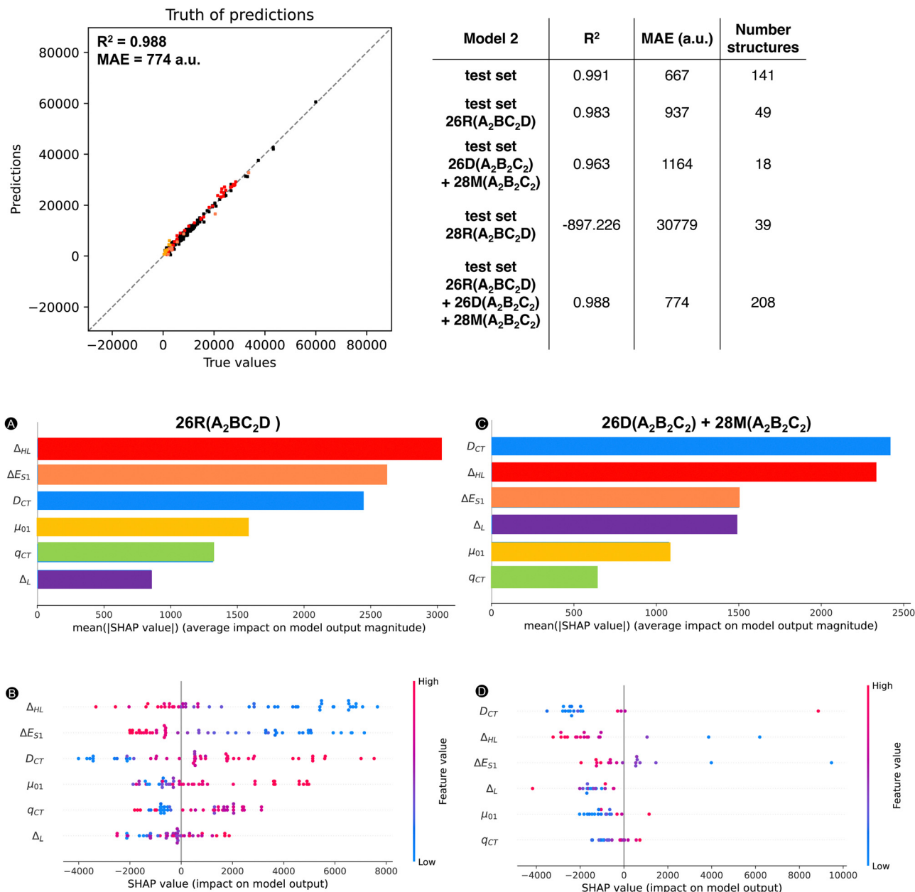
Fig. 14 Truth of predictions plot: scatter plot of true values ( i.e. \beta_{HRS} based on quantum chemical calculations) and predictions ( \beta_{HRS} predicted by model 2) on the initial test set, and new test sets 26R(A_2BC_2D) and 26D + 28M(A_2B_2C_2) with MAE and R^2 for the initial test set, the three extra test sets, and the total test set excluding the 28R (figure statistics). Below, SHAP analysis of the first two external test sets. (A) Bar plot containing the feature importances as the mean absolute SHAP value for each feature and all samples for 26R(A_2BC_2D) (B) bar plot containing the feature importances as the mean absolute SHAP value for each feature and all samples for 26D + 28M(A_2B_2C_2) (C) beeswarm plot with SHAP values of all data points while highlighting the feature value for 26R(A_2BC_2D) . (D) Beeswarm plot with SHAP values of all data points while highlighting the feature value for 26D + 28M(A_2B_2C_2) .
