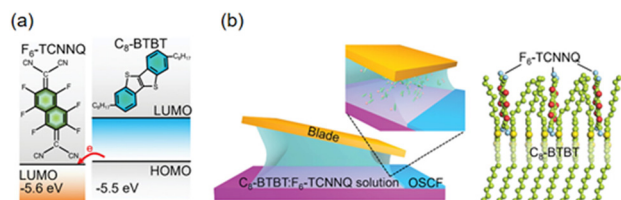
Fig. 5 (a) Chemical structures of C8-BTBT and F6-TCNNQ and schematic of charge transfer between C8-BTBT and F6-TCNNQ. (b) Schematic of solution deposition for anion-doped C8-BTBT thin films. Right: Distribution of F6-TCNNQ anions within the C8-BTBT thin film. Reprinted with permission from ref. 53. Copyright 2024, WILEY.
