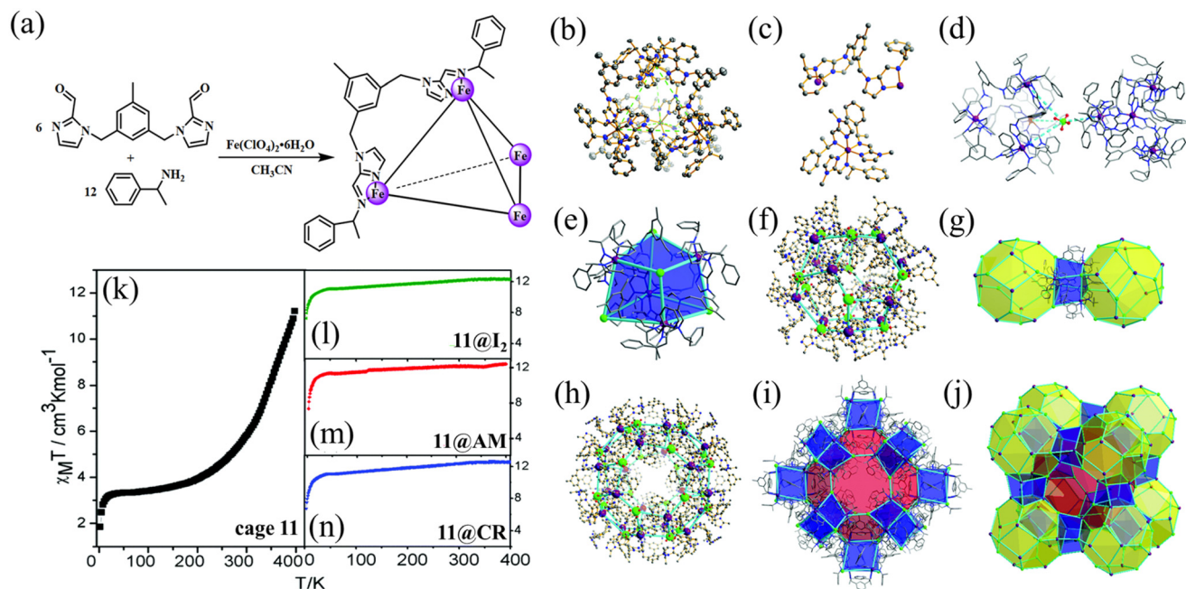
Fig. 11 Synthesis method (a) and crystal structure of cage 11. (b) (c) One edge and one vertex of cage 11. (d) Two adjacent cages bridged through a \text{ClO}_4^- anion. (e) Diagram of double 4-rings. (f) Diagram of \beta -cage. (g) Diagram of two \beta -cage attached to a double 4-rings. (h) Diagram of \alpha -cage. (i) Diagram of 12 double-4 rings around each \alpha -cage. (j) Diagram of LTA topology. \chi_m T vs. T plots for 11 (k), 11@I 2 (l), 11@AM (m) and 11@CR (n). 82
