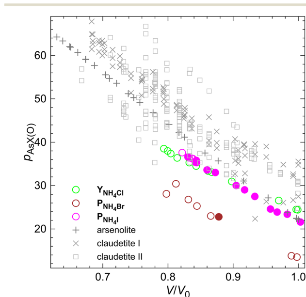
Fig. 4 Penetration indices of \text{As}\cdots\text{X} and \text{As}\cdots\text{O} secondary bonds in the studied intercalates and \text{As}_2\text{O}_3 polymorphs plotted as a function of V/V_0 unit-cell volume ratio. Data for arsenic(III) oxide polymorphs are taken from ref. 34–36.
