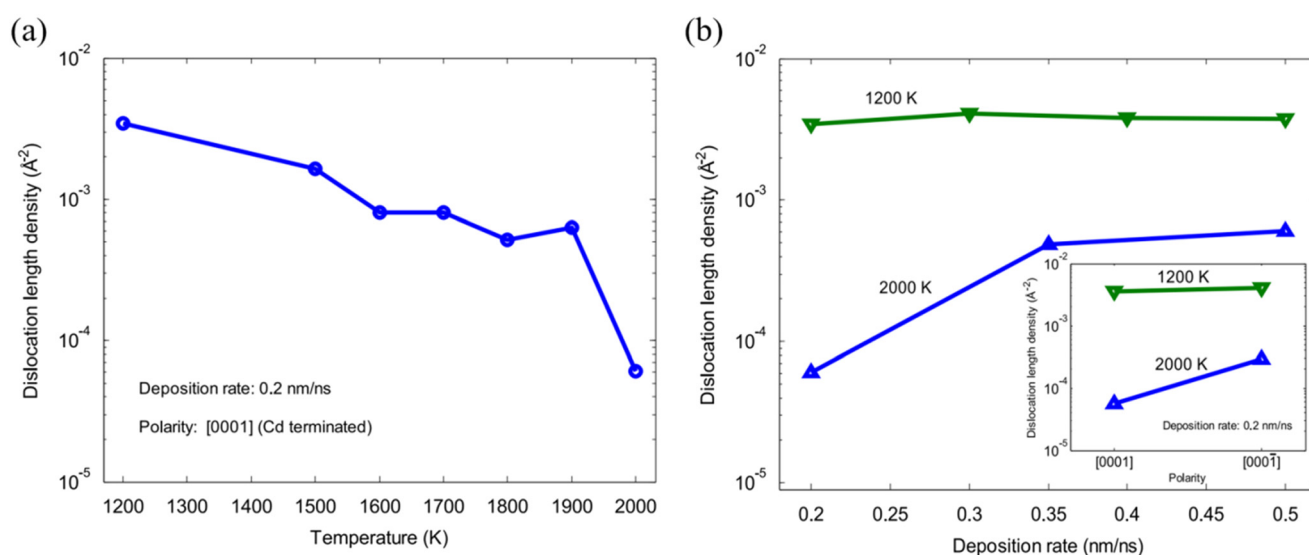
Fig. 4 (a) Dislocation length density as a function of substrate temperatures at constant deposition rate. (b) Dislocation length density as a function of different deposition rates at 1200\text{ K} and 2000\text{ K} . The inset shows the dislocation length density for different polarities: [0001] for Cd-terminated and [0001̄] for S terminated surfaces at 1200\text{ K} and 2000\text{ K} (copyright from Elsevier, Journal of Crystal Growth). 51
