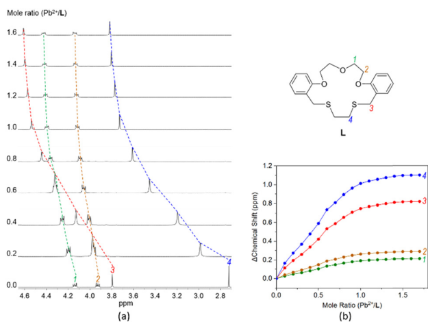
Fig. 3 (a) 1 H NMR titration of L (1.0 × 10 -3 M) with lead(II) perchlorate in CDCl 3 /CD 3 CN (v/v 1:1) and (b) titration curves for each proton in L .
