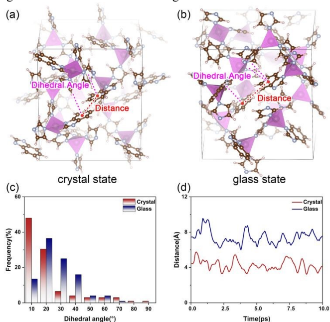
Figure 2 (a) Representation of the ZIF-62 crystal. (b) Snapshot of the simulated ZIF-62 glass. (c) The distribution of the dihedral angles between adjacent BIM ligands in two states. (d) The evolutions of the average distances between the centers of the benzene rings in the neighboring BIM ligands in two states. The analyzed dihedral angle and distance are marked in the above figures.
