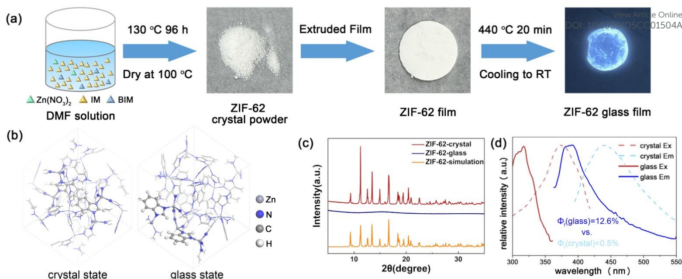
Fig. 1 (a) Experimental preparation process of ZIF-62 glass. (b) Crystalline and glassy structures. The closely packed and disordered ligands are highlighted using ball-and-stick model. (c) XRD patterns. (d) Absorption (Ex) and emission (Em) spectra of the ZIF-62 crystal and glass samples.
