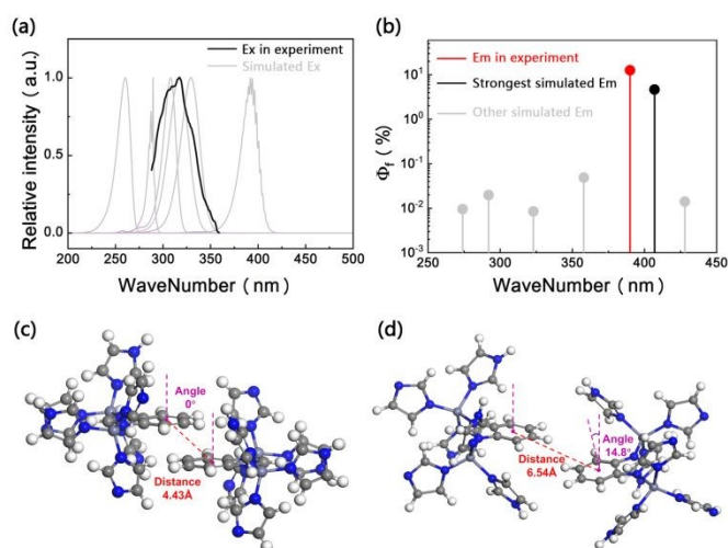
Fig. 3 (a) The simulated adsorption spectrum based on the cluster models. (b) The emission wavelengths of the examined configurations of the glassy state. (c) The arrangement of BIM ligands in the crystalline state. (d) The arrangement of BIM ligand in the configuration with the largest \Phi_f .
