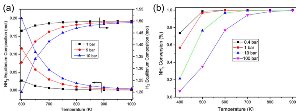
Fig. 3 (a) Equilibrium composition of ammonia and hydrogen product as a function of temperature, at constant pressures of 1, 5, and 10 bars, respectively (MATLAB's minimization of total Gibbs free energy) and (b) conversion of ammonia as a function of reaction temperature at different constant pressures. 14,49 (Reproduced from ref. 49, with permission from Springer Nature, copyright 2020).
