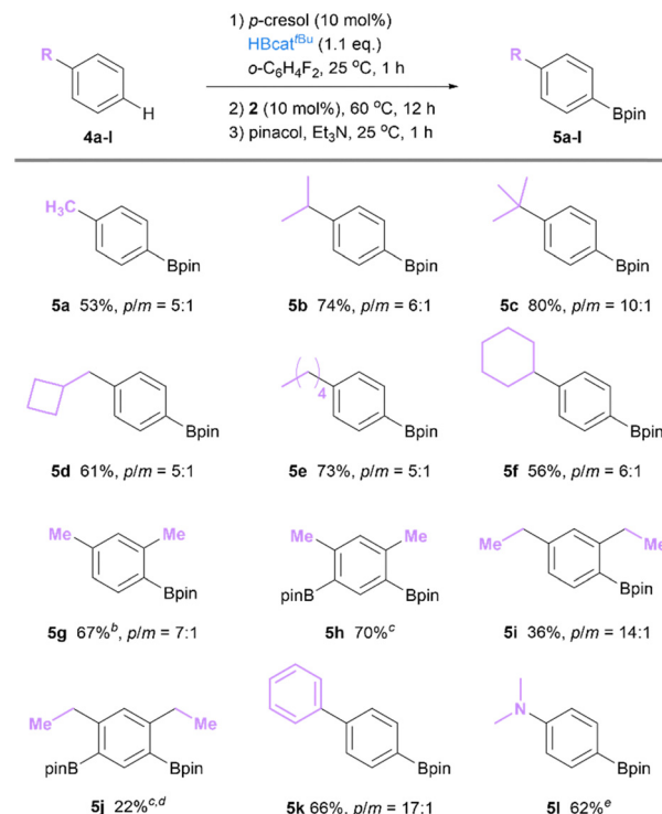
Scheme 2 Borylation of alkylarenes catalysed by 2. a 2 (10 mol%), p -cresol (10 mol%), arene (0.5 mmol), and HBcat tBu (0.55 mmol) in 0.6 mL of o -C 6 H 4 F 2 with isolated yields based on arenes. b 9% of 4,6-diborylated product was also obtained. c 2.5 equivalent of HBcat tBu was applied. d 17% of 5-monoborylated product was also obtained. e Without ( p -tol)OBcat tBu additive.
