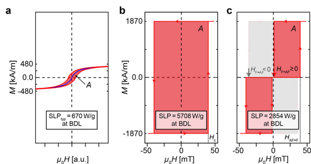
Fig. 1 Physics-based limits of specific loss parameters under the boundary conditions of the biological discomfort level. (a) M(H) -loop of a superparamagnetic nanoparticle particle showing Langevin-like loop without hysteresis for slowly varying fields (blue curve) and developing a small hysteretic loss (red-shaded area) for fields oscillating at higher frequencies. (b) Ideal M(H) -loop of a ferromagnetic disk particle (F-MDP) leading to the largest hysteretic loss (red-shaded area) of 5708 \text{W g}_{\text{CoFe}}^{-1} possible under consideration of the biological discomfort level. (c) Ideal M(H) -loop of a synthetic antiferromagnet (AF) disk particle (SAF-MDP) with m(H = 0) = 0 (red-shaded area). The maximum SLP is half the size of that of the F-MDP, but can be increased for a SAF-MDP with a reduced antiferromagnetic (AF) coupling (light gray shaded additional area). Then the magnetic moment does not longer vanish at zero field, and a demagnetization procedure has to be applied to re-set the SAF-MDP into its AF-coupled ground state.
