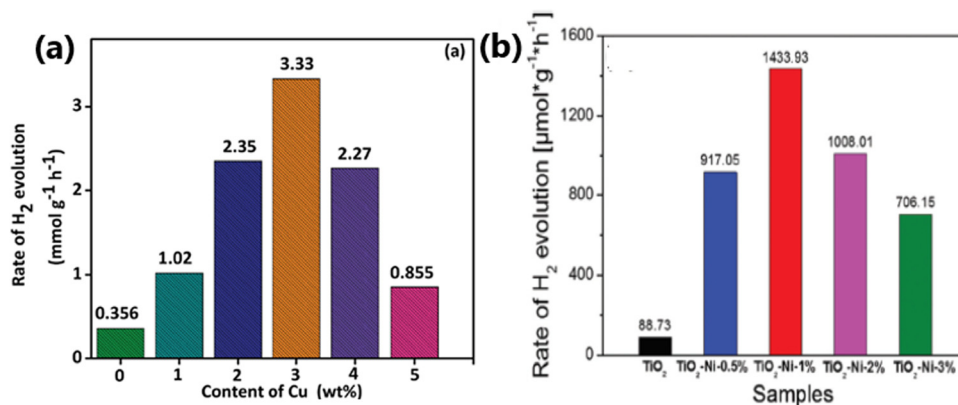
Fig. 26 (a) Variation in the \text{H}_2 evolution activity of \text{TiO}_2 decorated with different wt% of Cu. Reproduced with permission from ref. 104. Copyright © 2017, the Royal Society of Chemistry. (b) Rate of hydrogen evolution of \text{TiO}_2 and TiNi samples with different loadings of Ni. Reproduced with permission from ref. 16. Copyright © 2018, the Royal Society of Chemistry.
