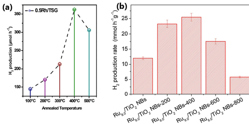
Fig. 20 (a) Variation in the rate of hydrogen production on 50 mg of 0.5Rh/TSG( \text{TiO}_2 ) as a function of calcination temperature (reproduced with permission from ref. 51. Copyright ©2018 Elsevier Ltd). (b) Variation in the rate of hydrogen production as a function of calcination temperature for the Ru (wt% = 8.0)/ \text{TiO}_2 NB photocatalyst (reproduced with permission from ref. 47. Copyright ©2016, Wiley-VCH).
