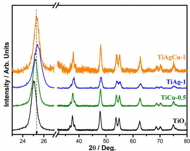
Fig. 1 Wide angle XRD patterns of mesoporous \text{TiO}_2 , \text{Ag/TiO}_2 (TiAg-1), \text{Cu/TiO}_2 (TiCu-0.5) and TiAgCu-1 nanocomposites. A significant shift and broadening of the (101) diffraction feature is observed with TiAg-1 and TiAgCu-1. All the diffraction features are attributed to the anatase phase of \text{TiO}_2 .
