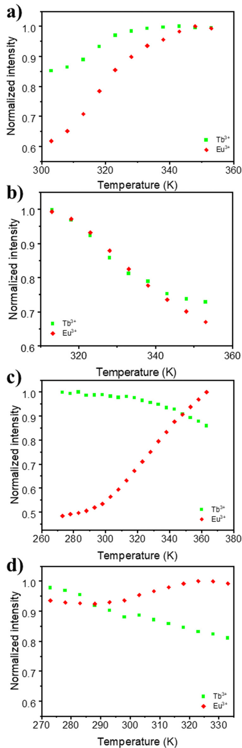
Fig. 5 Thermal evolution of the integrated emission intensity of the exchanged analogues: (a) UCY-17( \text{Eu}_{0.05}\text{Tb}_{0.95} )/BDC, (b) UCY-17( \text{Eu}_{0.05}\text{Tb}_{0.95} )/ABDC, (c) UCY-17( \text{Eu}_{0.05}\text{Tb}_{0.95} )/FBDC, and (d) UCY-17( \text{Eu}_{0.05}\text{Tb}_{0.95} )/NDC.
