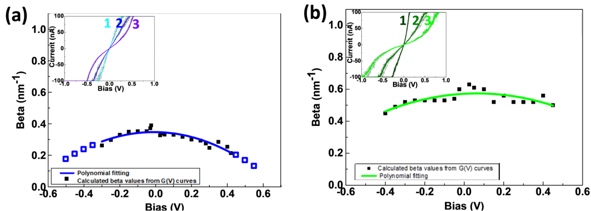
Fig. 6 Attenuation factor \beta_v versus voltage of (a) Au-[CoTPP] n -Au and (b) Au-[TPP] n -Au SMJs calculated from I/V curves (for three different lengths, inset images). Black square points are extrapolated values from I/V curves at different bias voltages.
