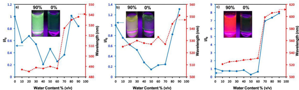
Fig. 19 Changes in the PL intensity and k_{\max} in THF–water mixtures with f_w = 10 – 90\% : (a) compound 24 , (b) compound 25 and (c) compound 26 . Inset: Fluorescence images of the luminogens in THF–water mixtures at f_w = 90\% and f_w = 0\% under illumination with a 365 nm UV lamp. Reproduced with permission from ref. 87. Copyright 2021 Elsevier.
