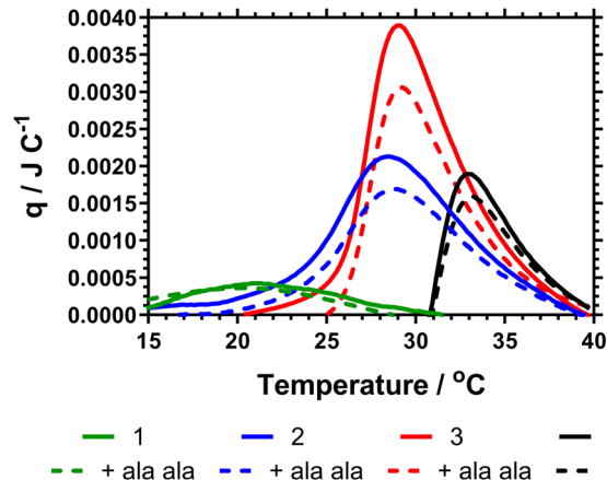
Fig. 4 Micro-DSC thermogram for HB-PNIPAM-Vanc in absence (solid lines) and presence (dashed lines) of D-Ala–D-Ala peptide in PBS. Contains vanc. functionalised polymers with 1 (DB 0.107 (green)), 2 (DB 0.038 (blue)), 3 (0.021 (red)) and 4 (linear polymer (black)).
