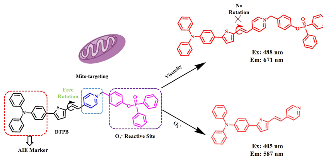
Fig. 3 Representative scheme of viscosity responsiveness by the triphenylamine-based AIE probe. 25 [Reproduced from Analytica Chimica Acta , 1253 , Wei Liu, Yan Wang, Tengfei Wang, Liwen Wang, Sheng Hu, Dating Tian, A versatile AIE probe with mitochondria targeting for the dual-channel detection of superoxide anion and viscosity, 341099., Copyright (2023), with permission from Elsevier].
