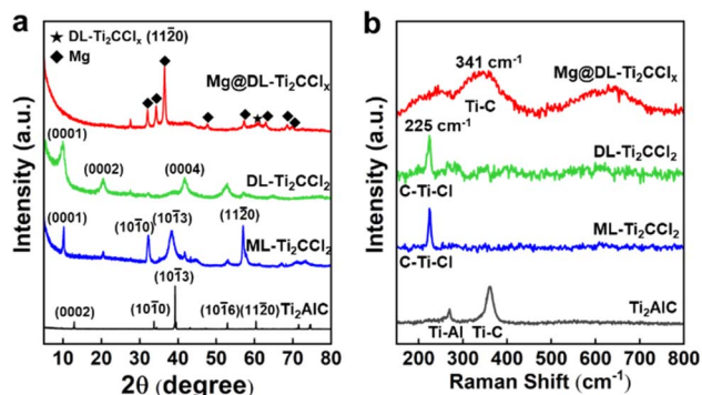
Fig. 2 Change of the crystalline and chemical structures of the Ti 2 AlC MAX phase, ML-Ti 2 CCl 2 , DL-Ti 2 CCl 2 and Mg@DL-Ti 2 CCl x composite based on (a) X-ray diffraction (XRD) patterns and (b) Raman spectra.
