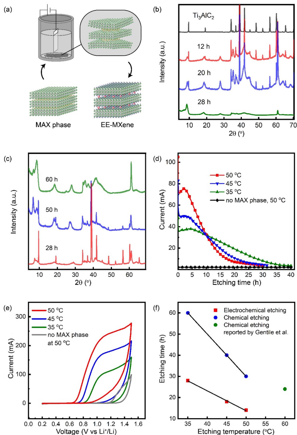
Fig. 1 (a) Schematic illustration of the setup. (b) XRD of \text{EE-Ti}_3\text{AlC}_2 etched with an applied voltage of +1 V at 35 °C with different etching times. (c) XRD pattern of \text{CE-Ti}_3\text{AlC}_2 at 35 °C with different etching times. (d) Amperometric monitoring of the electrochemical etching of \text{EE-Ti}_3\text{AlC}_2 at various temperatures. (e) Cyclic voltammetry curve of 1 g of \text{Ti}_3\text{AlC}_2 at various temperatures. Scan rate: 10 \text{ mV s}^{-1} . (f) Etching time required to completely etch \text{Ti}_3\text{AlC}_2 to \text{Ti}_3\text{C}_2 by electrochemical etching and electrochemical etching at various temperatures.
