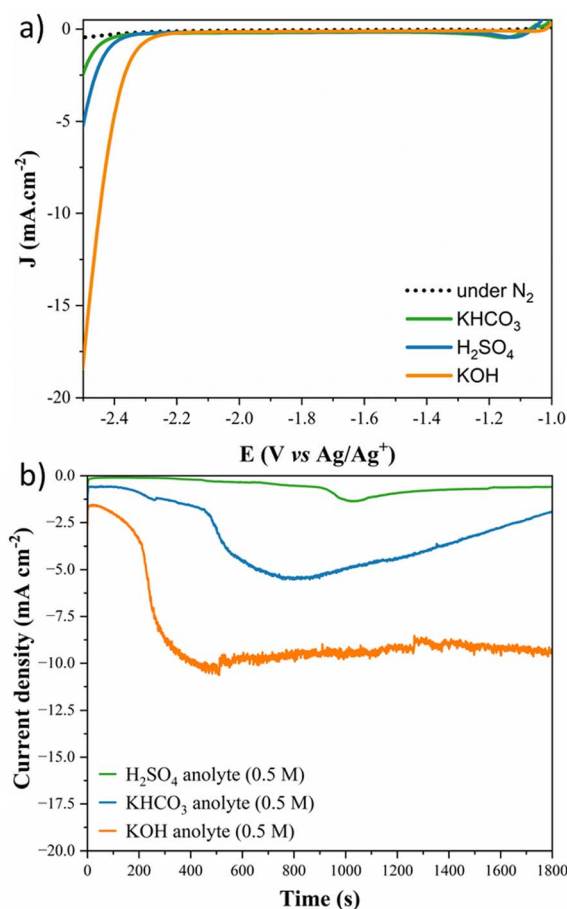
Fig. 1 (a) CO_2 RR polarization curve for a Pb plate electrode in dried acetonitrile 0.1 M TBAPF 6 with H_2SO_4 , KHCO_3 , and KOH anolytes and (b) chronoamperometric curve for the different anolytes on the Pb plate.
