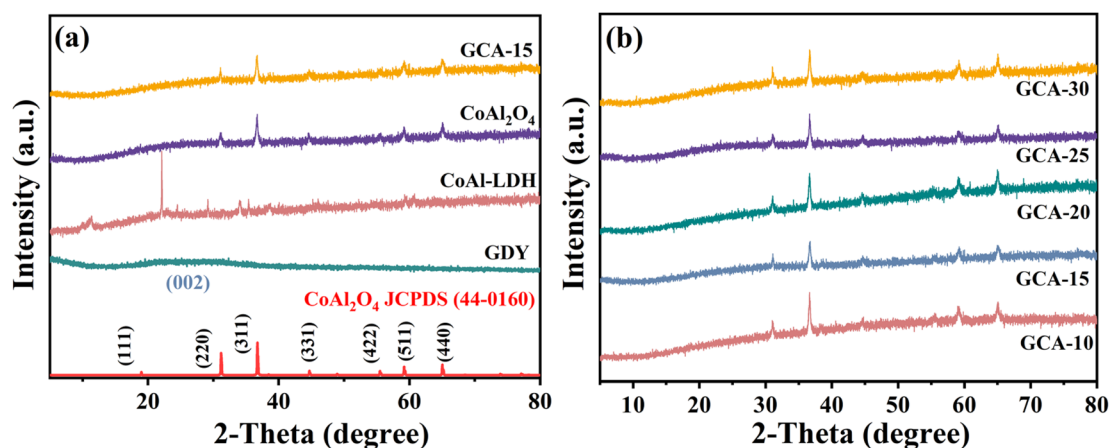
Fig. 2 (a) XRD patterns of GDY, precursor CoAl-LDHs, annealed CoAl 2 O 4 and GCA-15; (b) GCA-X samples.
