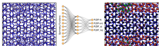
Fig. 3 Schematics of our neural network trained over atom-centred symmetry functions of ZIF-4, ZIF_a, ZIF-zni and ZIF_liq microstates that allows the classification of \text{Zn}^{2+} -centred environments. Left and right hand illustrations: before and after the classification (colour code: ZIF-4- (black), ZIF_liq- (orange) and ZIF_a-like environments (green).
