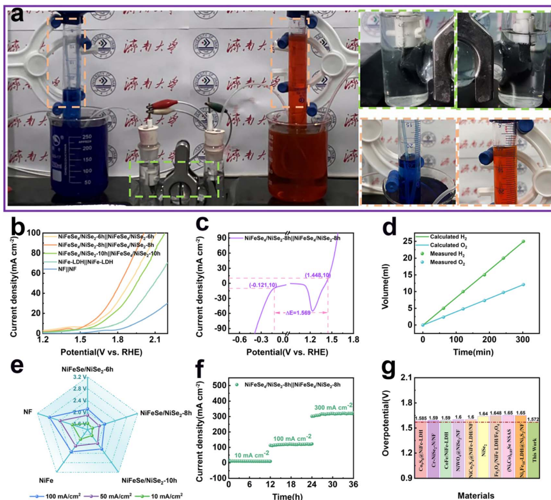
Fig. 7 Overall water splitting performance of different materials in the double-electrode system: (a) the \text{NiFeSe}_4/\text{NiSe}_2-8\text{ h}||\text{NiFeSe}_4/\text{NiSe}_2-8\text{ h} double-electrodes system for overall water splitting and gas collection; (b) polarization curves; (c) \text{NiFeSe}_4/\text{NiSe}_2-8\text{ h} LSV curves for the OER and HER; (d) the volumes of \text{H}_2 and \text{O}_2 experimentally measured and theoretically calculated versus time at 20\text{ mA cm}^{-2} ; (e) different current densities corresponding to overpotential; (f) stability test; (g) comparison with other overall water splitting works.
