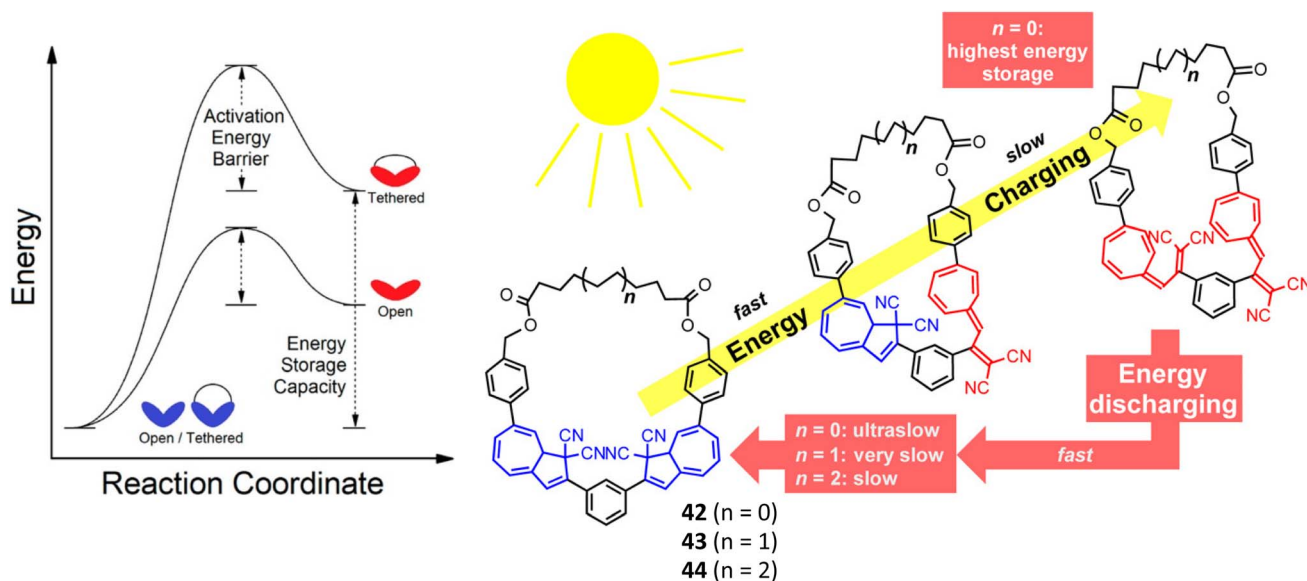
Figure 17 Left: Simplified potential energy surface for acyclic and cyclic, dimeric systems converting between DHA–DHA (blue) and VHF–VHF (red) isomers. Right: Macrocyclic DHA dimers studied by Mikkelsen and Nielsen et al. with various ring sizes. 88 Figures reproduced from ref. 88 with permission from the American Chemical Society.
