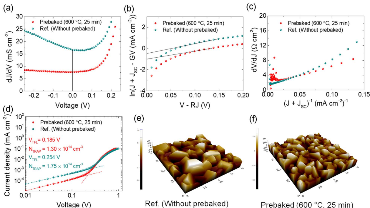
Fig. 4 Dark J - V behavior of the prebaked and W.B. film-based devices. (a) Shunt conductance, (b) reverse saturation current, (c) series resistance with ideality factor, (d) full logarithmic characteristics of the J - V curve, and (e and f) AFM topography of the ref. and prebaked source films.
