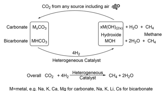
Fig. 1 CO 2 capture with a metal hydroxide and hydrogenation of the obtained carbonate/bicarbonate to methane with concurrent recycling of the base.
