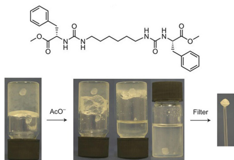
Fig. 41 Structure of a urea-based gelator used to control API crystallisation and photographs of the growth of a crystal of carbamazepine within the gel, and the use of acetate anions to disassemble the gel and allow recovery of the crystal. Figure reproduced from ref. 331 with permission of Springer Nature, © 2010.
