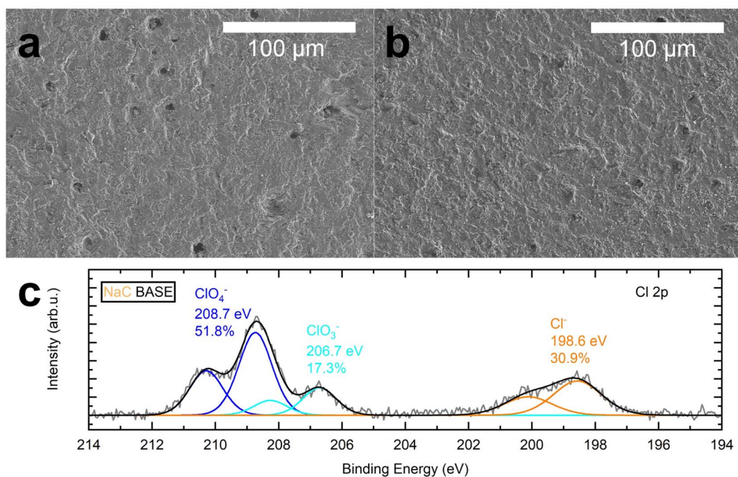
Fig. 4 SEM and XPS analysis of the sodium-β alumina solid electrolyte (BASE). (a) SEM image of a pristine BASE surface. (b) Post-mortem SEM image of a BASE that had been in contact with NaC and the cathode. (c) Post-mortem XP spectrum of BASE's Cl 2p core level. The BASE had been in contact with NaC and the cathode.
