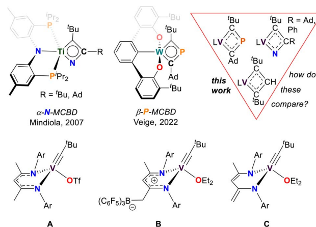
Fig. 1 Top: Isolable pnictogen-based metallacyclobutadienes (MCBD) complexes and the vanadacyclobutadiene (VCBD) species reported in this work ( L = dBDI^{2-} ). Bottom: Selected [V^V] alkyldiyne complexes, with complex C being the focus of the present study.
