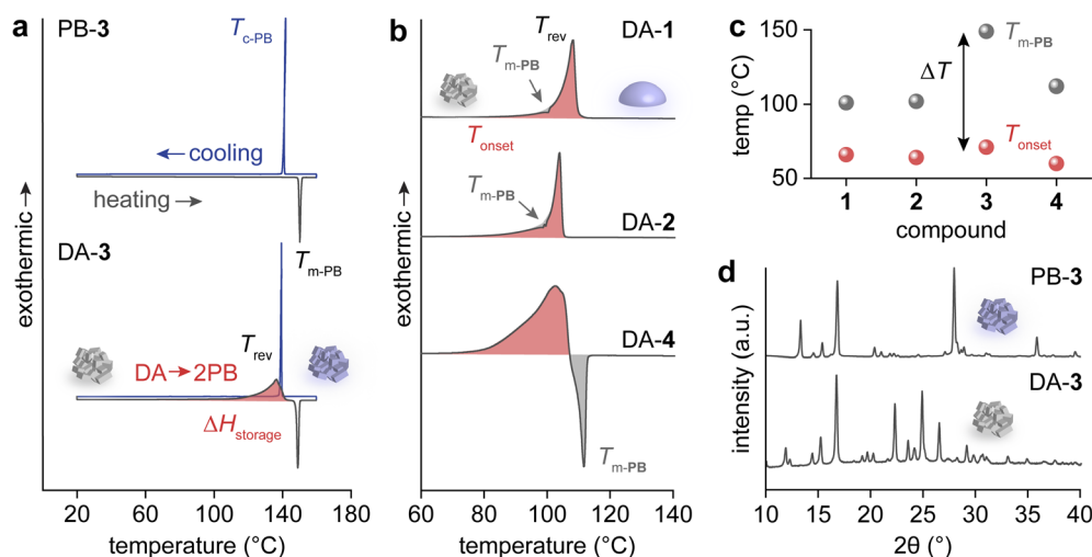
Fig. 2 (a) DSC thermograms of PB-3 and DA-3 measured during the first heating (black) and cooling (blue) cycle. (b) DSC thermograms of DA-1, DA-2, and DA-4, measured during the first heating cycle. (c) Relative T_{m-PB} and T_{onset} of compounds 1–4. (d) PXRD patterns of PB-3 and DA-3. Red highlighted areas represent the exotherms of cycloreversion ( \Delta H_{storage} ). Grey highlighted areas represent the endotherms of melting of phenylbenzoxazole; T_{m-PB} , melting point of phenylbenzoxazole; T_{c-PB} , crystallization point of phenylbenzoxazole; T_{rev} , peak temperature of thermal reversion; T_{onset} , onset temperature of thermal reversion; \Delta T , difference between T_{m-PB} and T_{onset} .
