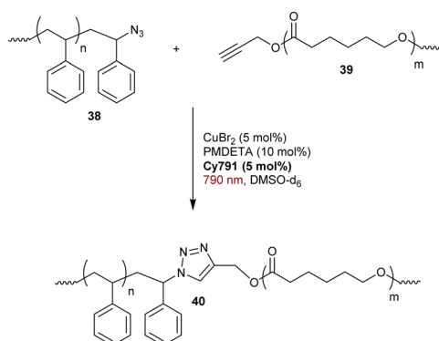
(a) Synthesis of PS- \beta -PCL block copolymer using Cy791 and NIR-Photoinduced CuAAC
