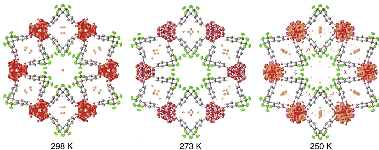
Fig. 4 Residual electron density within \text{CF}_4 -dosed \text{Zn(fba)} . A crystal of \text{Zn(fba)} housed within a borosilicate capillary was dosed with 1 bar \text{CF}_4 at ambient temperature, flame sealed, and mounted onto a diffractometer goniometer head. Data collection was performed at 298 K, 273 K, and 250 K. The capillary was allowed to equilibrate for at least 2 h at the analysis temperature prior to data collection. Orange and red regions correspond to positive and negative residual density, respectively. Electron density maps were generated using the Olex2 software package. 51 Isosurface values are set at 0.28 \text{ e } \text{\AA}^{-3} .
