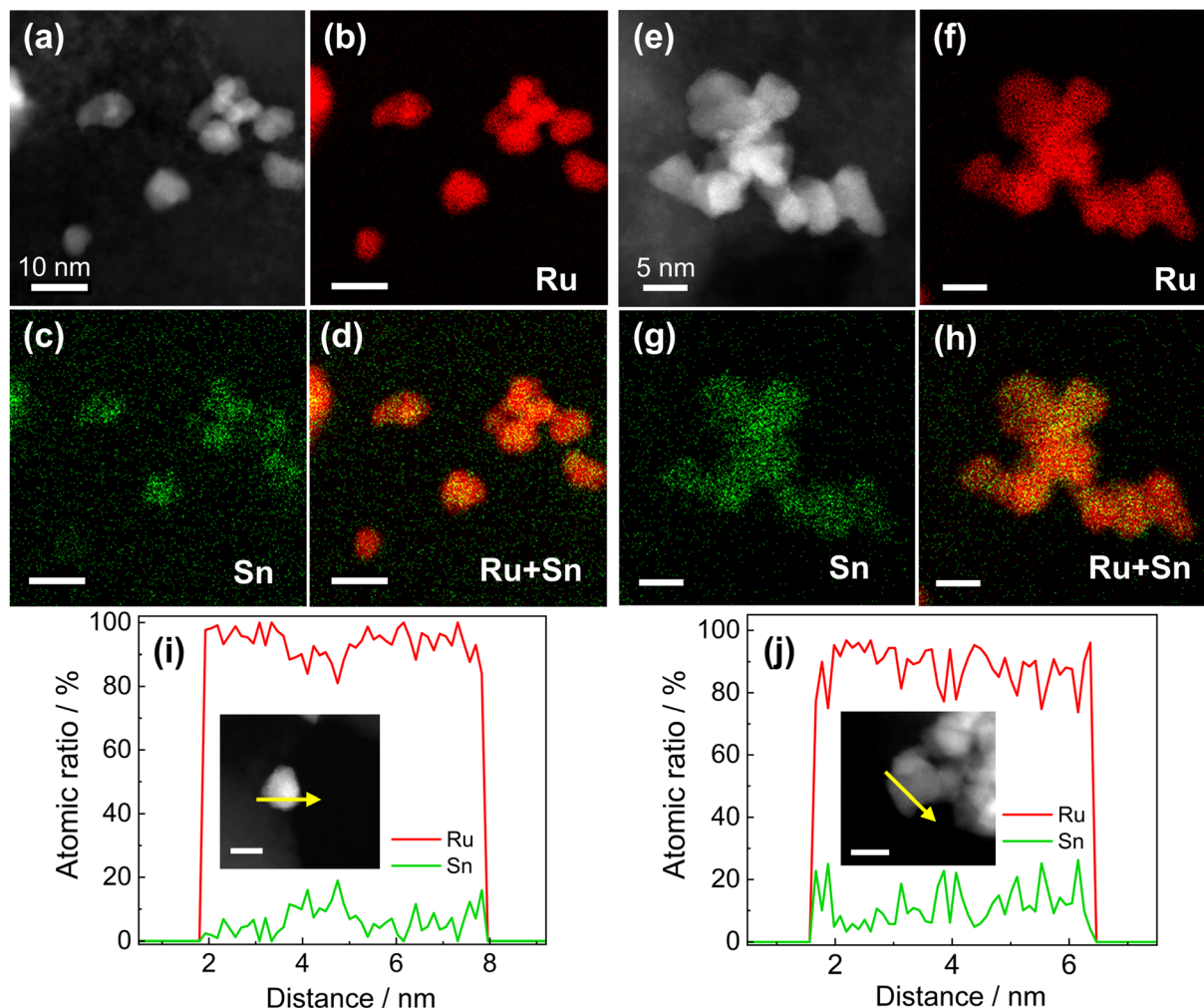
Fig. 1 (a) HAADF-STEM image of Ru 0.94 Sn 0.06 NPs/C. STEM-EDX elemental mapping of Ru 0.94 Sn 0.06 NPs/C showing (b) Ru (L-line), (c) Sn (L-line) and (d) overlay images. (e) HAADF-STEM image of Ru 0.87 Sn 0.13 NPs/C. STEM-EDX elemental mapping of Ru 0.87 Sn 0.13 NPs/C showing (f) Ru (L-line), (g) Sn (L-line) and (h) overlay images. EDX line scan profiles of (i) Ru 0.94 Sn 0.06 NPs/C and (j) Ru 0.87 Sn 0.13 NPs/C. The arrow in the inset indicates the direction of the line scan. The scale bar in the inset is 5 nm.
