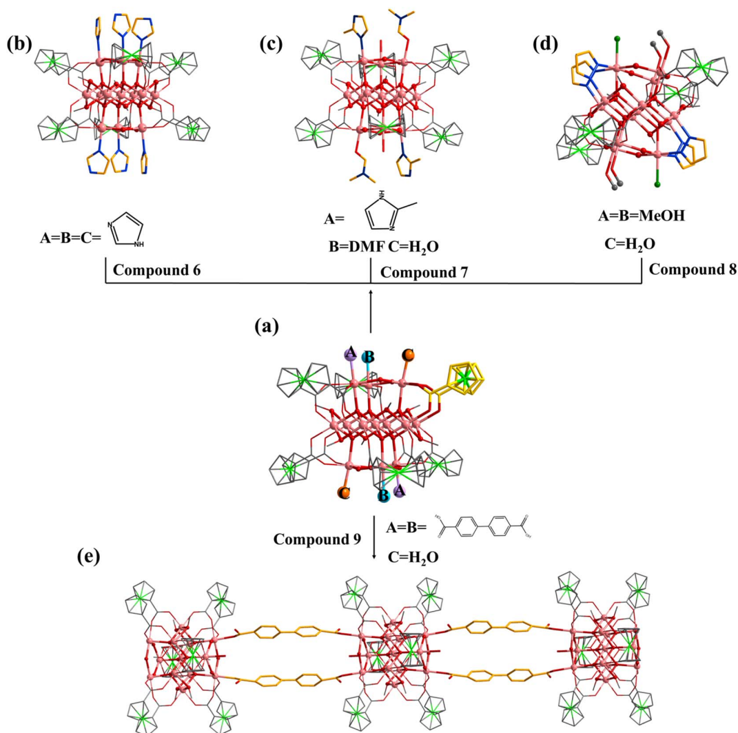
Fig. 5 (a) [\text{In}_{13}] as a secondary building unit; (b) compound 6 ( A = B = C = \text{HIm} ); (c) compound 7 ( A = \text{2-mim} , B = \text{DMF} , C = \text{H}_2\text{O} ); (d) compound 8 ( A = B = \text{MeOH} , C = \text{H}_2\text{O} ); (e) compound 9 ( A = B = \text{BPDC} , C = \text{H}_2\text{O} ). A, B and C represent different substitution sites.
