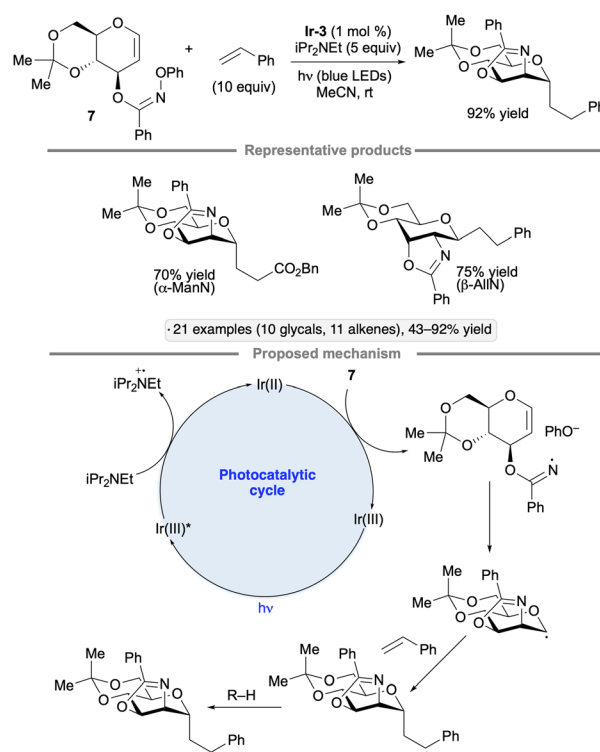
Scheme 46 Photocatalytic process for net aminoalkylation of glycals via anomeric radicals. Ir-3 denotes [Ir(ppy)_2(dtbbpy)]PF_6 .
