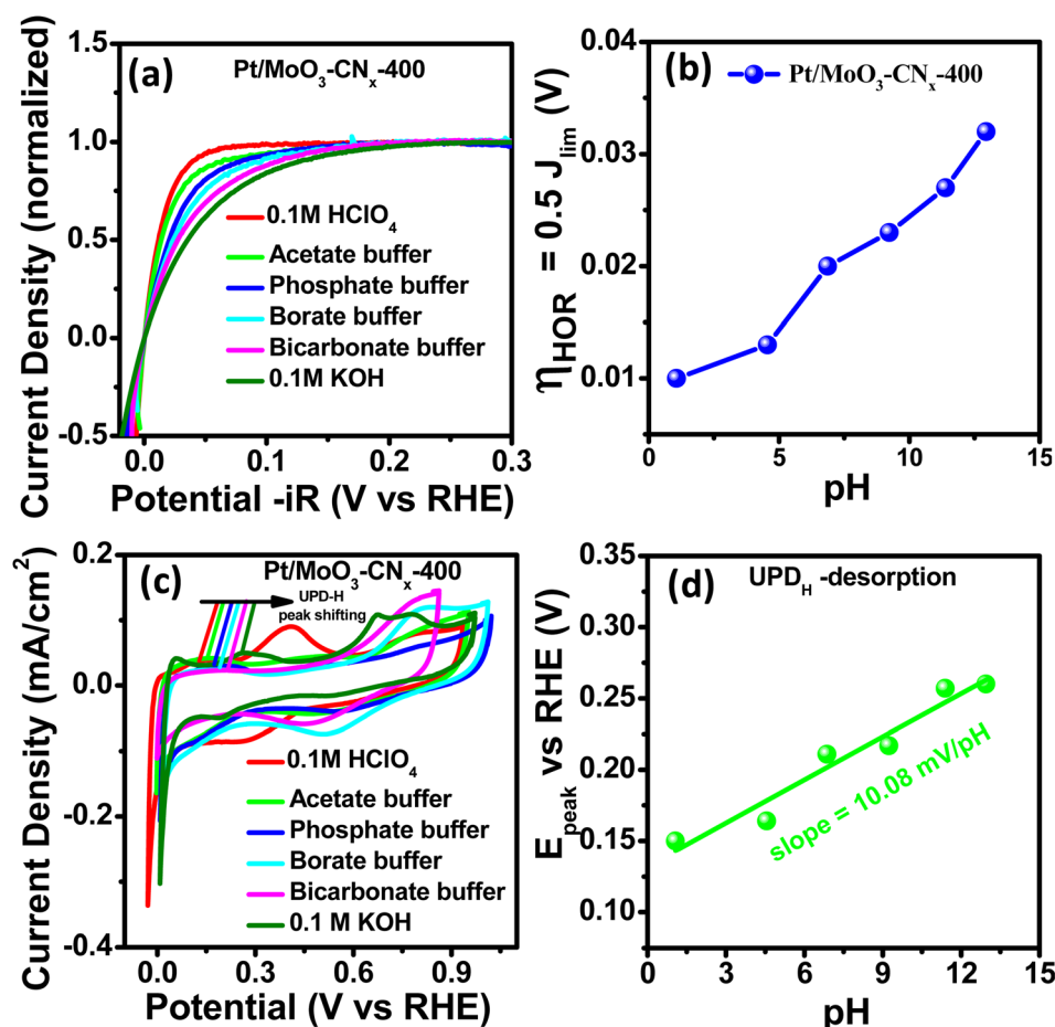
Fig. 5 (a) Normalized HOR plots for Pt/MoO 3 -CN x -400 in different pH solutions. (b) Overpotential at 0.5 × J_{lim} vs. pH plot of the catalyst. (c) CV curves for Pt/MoO 3 -CN x -400 in different pH solutions. (d) E_{peak} of UPD-H vs. pH plot of Pt/MoO 3 -CN x -400.
