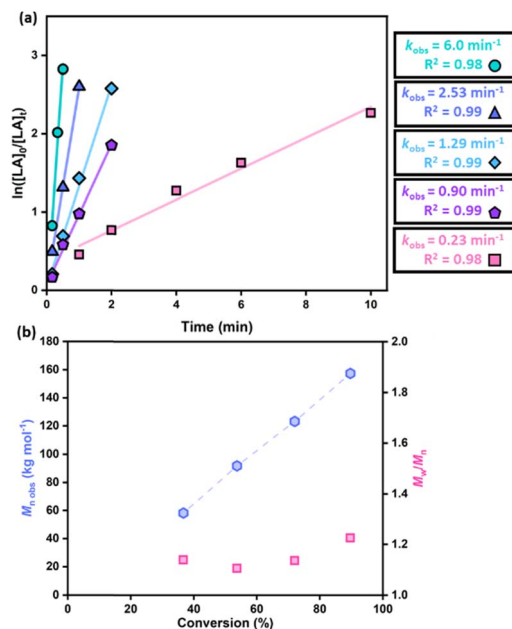
Fig. 2 (a) Semi-logarithmic plot of rac -LA conversion vs. time at 70 °C with Zn(OBn)_2 in toluene solvent with various [cat]:[ rac -LA] loading ratios ( [rac-LA] = 1 \text{ M} for 1:100 (circles); 1:300 (triangles); 1:500 (diamonds) and 1:1000 (pentagon) loadings, and 2 M for 1:2500 (square) loadings), with k_{obs} and R^2 values presented in the figure legend. (b) Evolution in M_n and M_w/M_n with monomer conversion for a [Zn(OBn)_2]:[rac-LA] ratio of 1:2500 ( [rac-LA] = 2 \text{ M} ) (refer to ESI, Fig. S4,† for additional plots of M_n vs. M_w/M_n ).
