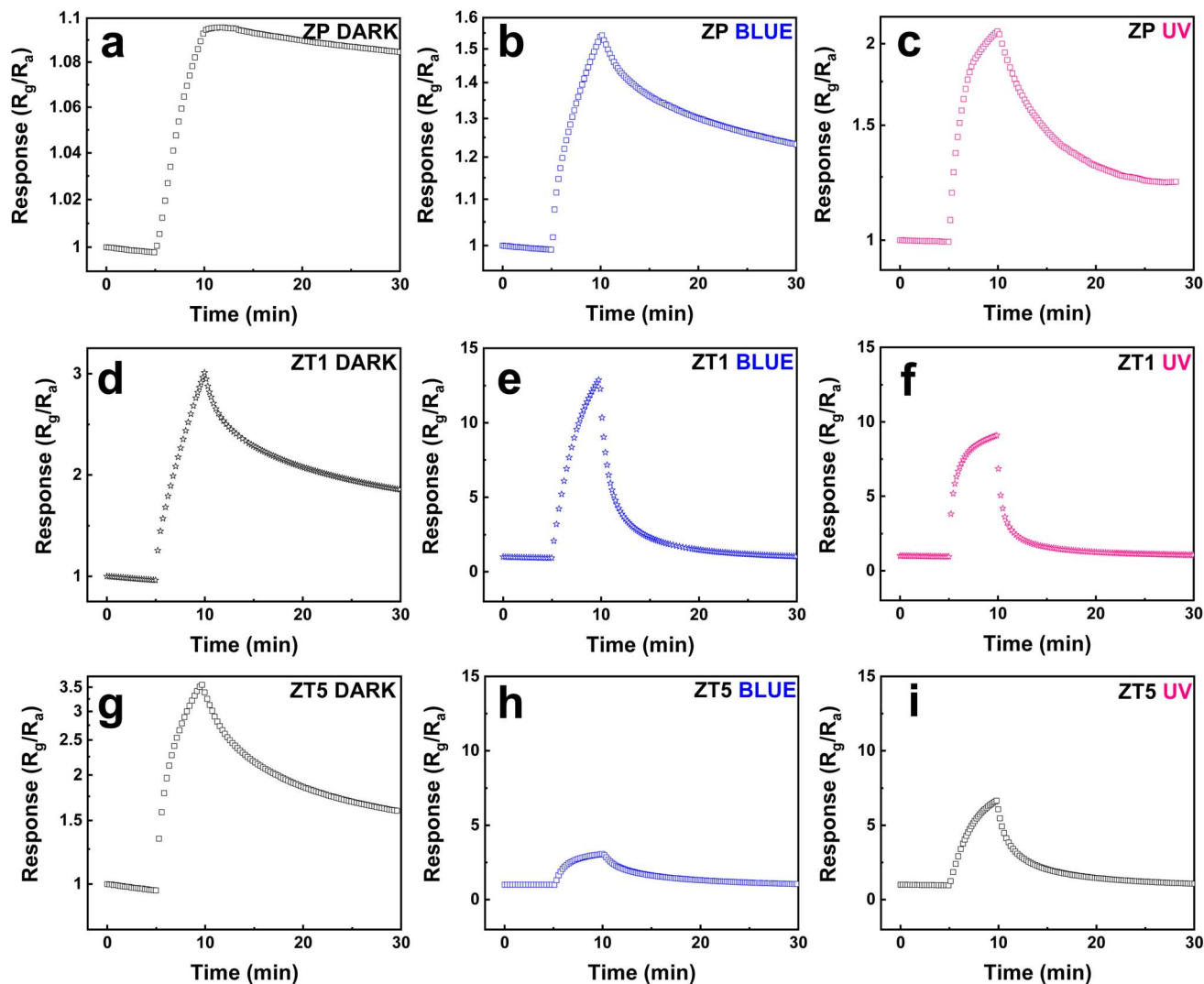
Fig. 5 Response curves to 500 ppb NO 2 of (a–c) ZP, (d–f) ZT1, (g–i) ZT5 under dark, blue, and UV irradiation sources.
